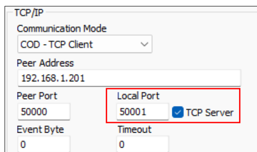
Fig 5.5-3 ezManager TCP Client 設定欄 2
