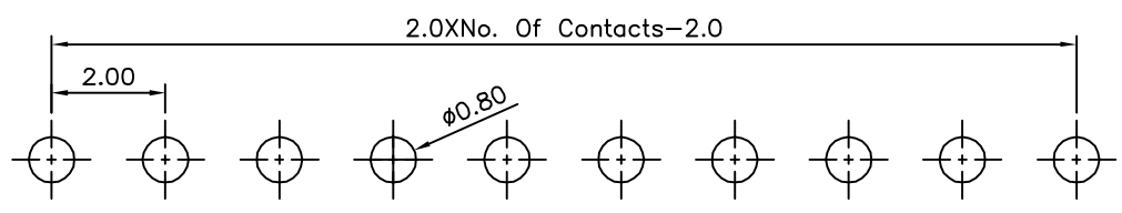
Recommended P.C.B. Layout
